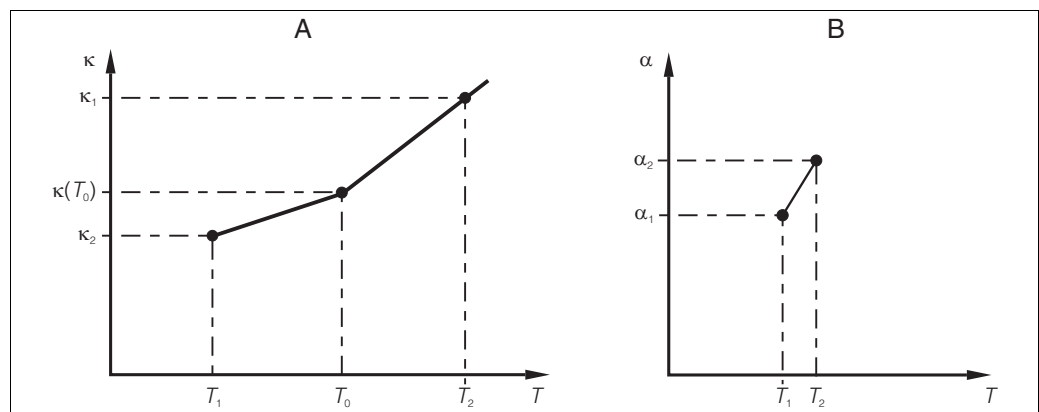
Fig. 24: Determination of temperatur coefficient
