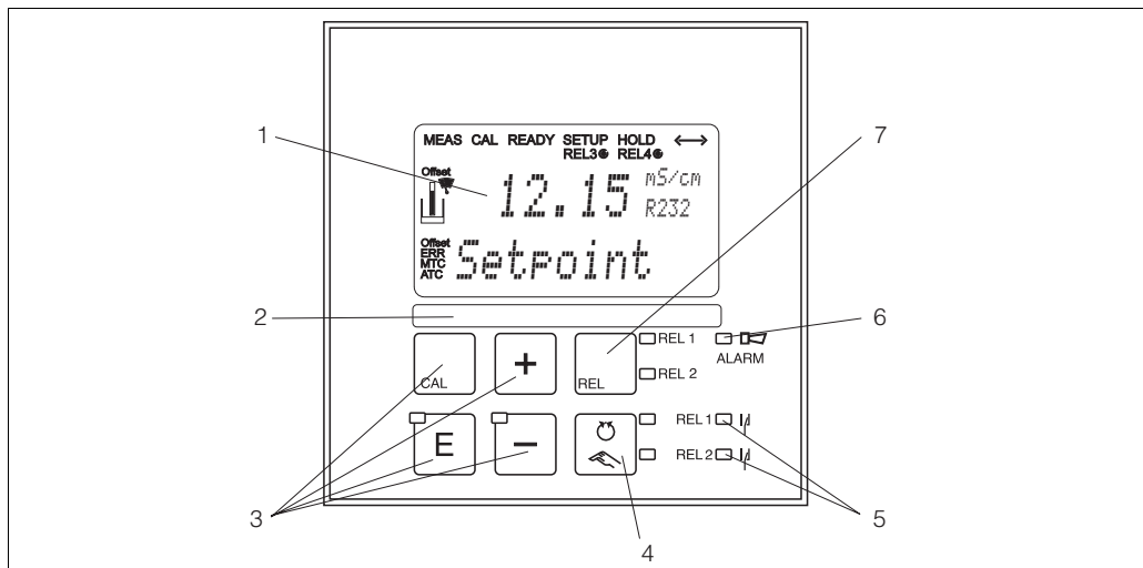
Fig. 17: Operating elements
