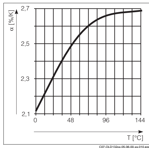
Fig. 23: NaCl compensation
