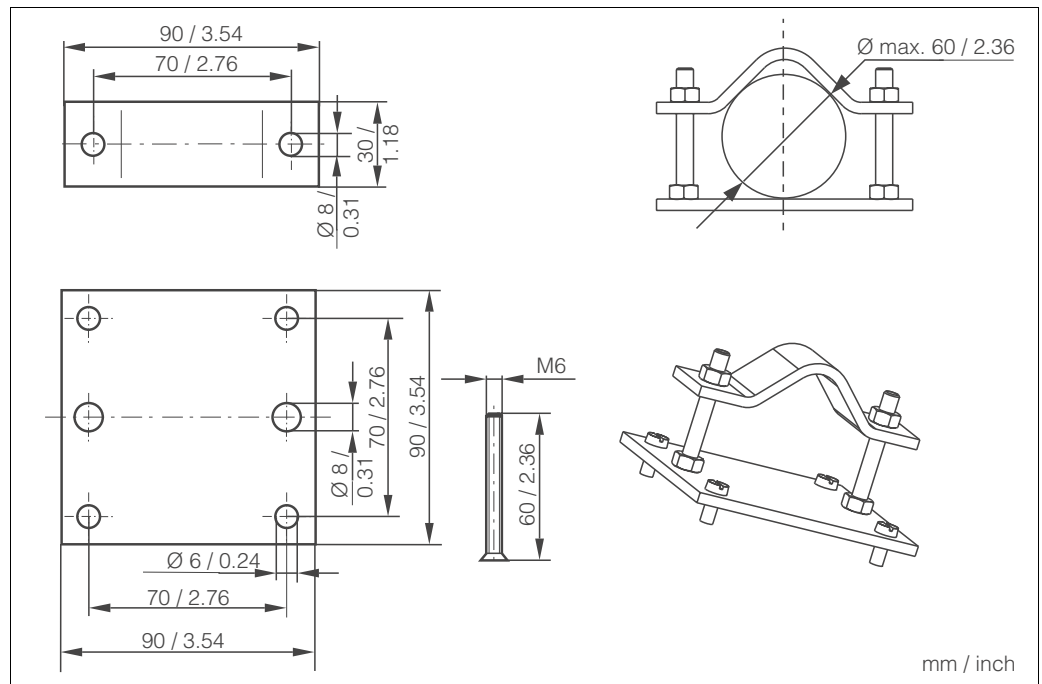
Fig. 41: Pipe mounting kit
