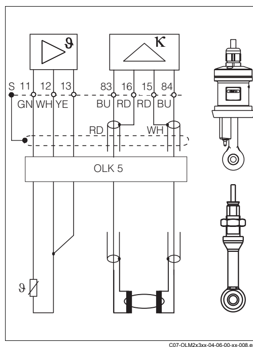
Fig. 14: Connection of inductive sensors
