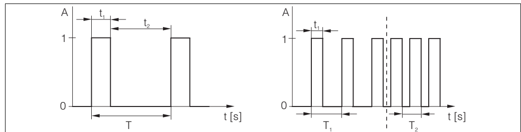
Fig. 32: Signal of a pulse-length modulated controller contact (left) and of a pulse-frequency modulated controller contact (right)
