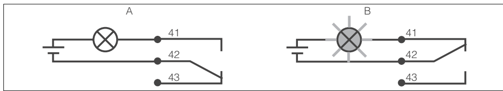
Fig. 15: Recommended fail-safe switching for the alarm contact
