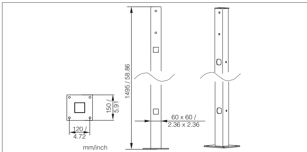
Fig. 40: Square post OYY102
