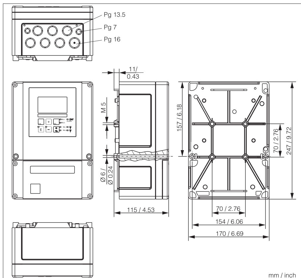
Fig. 2: Field instrument
