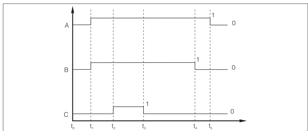
Fig. 35: Sequence of a cleaning cycle
