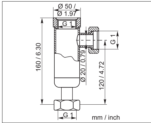
Fig. 43: OLA751 flow assembly
