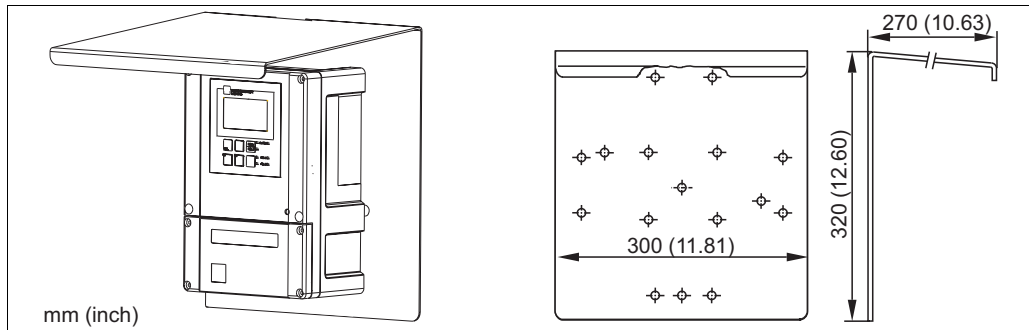
Fig. 39: Weather protection cover for field instrument
