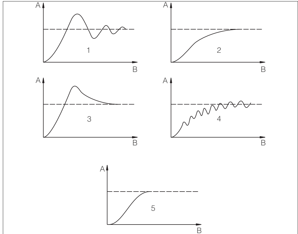
Fig. 31: Optimisation of settings T_n and K_p
