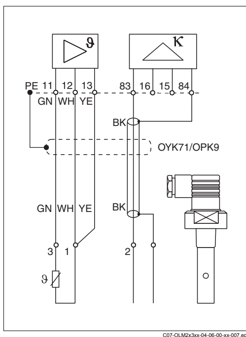
Fig. 13: Connection of conductive sensors
